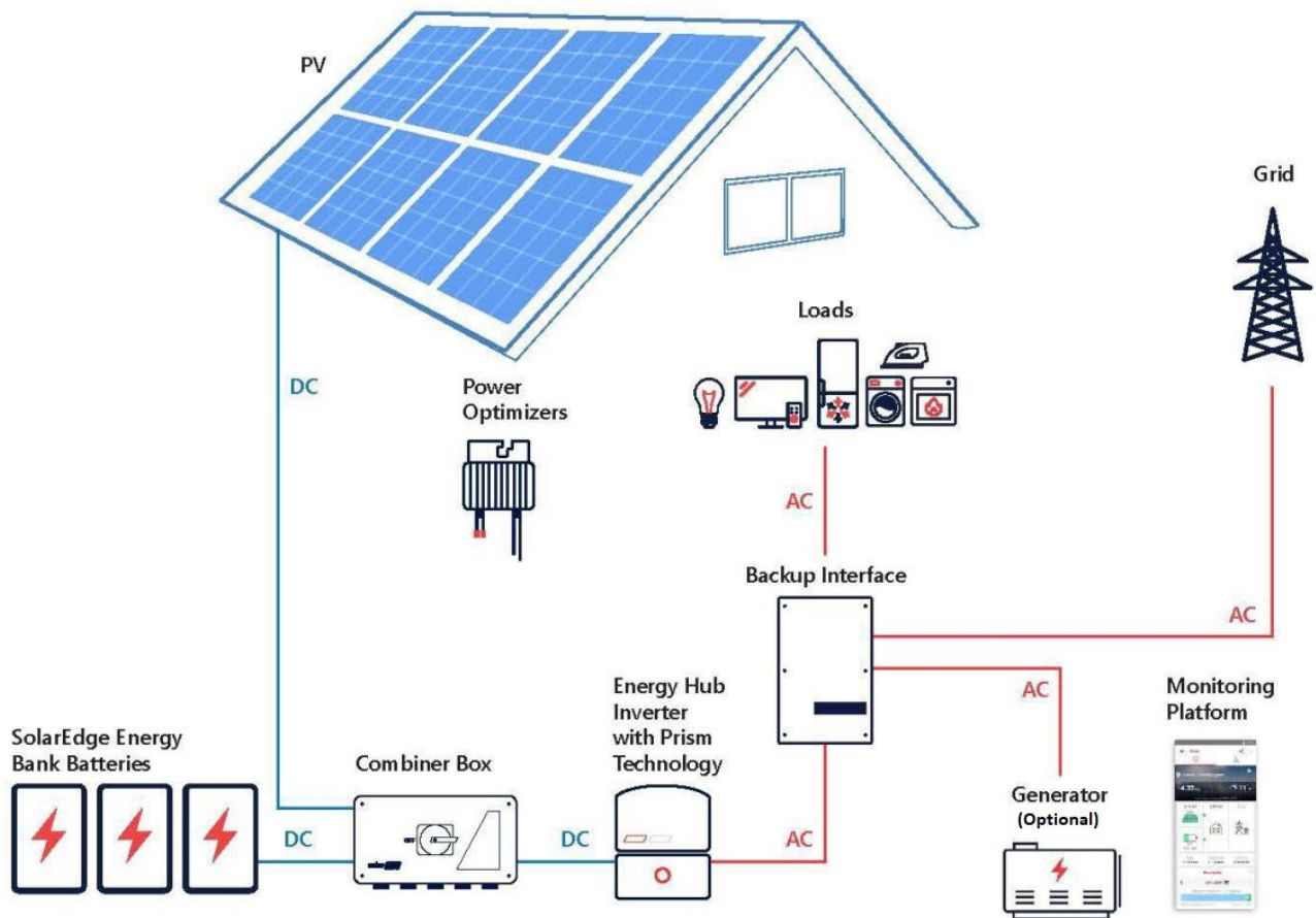
Figure 1 System Overview – Complete PV and Battery With Backup System
